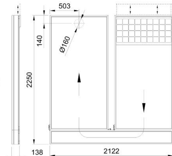
TWINSOLAR compact 4.5
